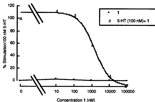
Figure 2. Effects of O -methylasparvenone ( 1 ) on the IP 3 formation in the rat choroid plexus.
